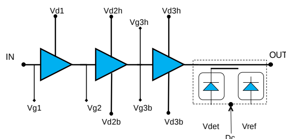
Functional diagram
