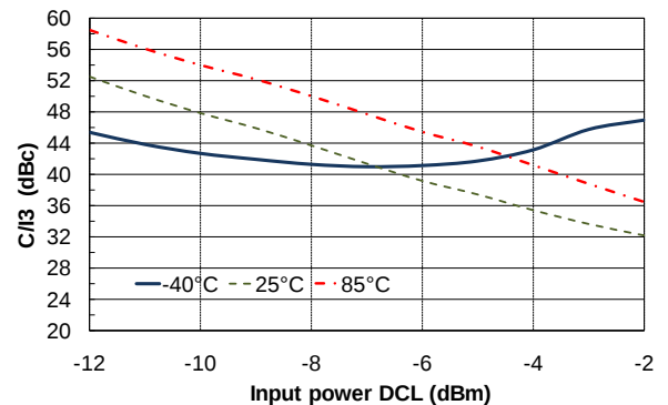
C/I3 versus input power and Temperature at 15GHz
