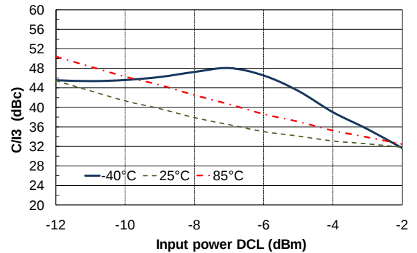
C/I3 versus input power and Temperature at 9GHz
