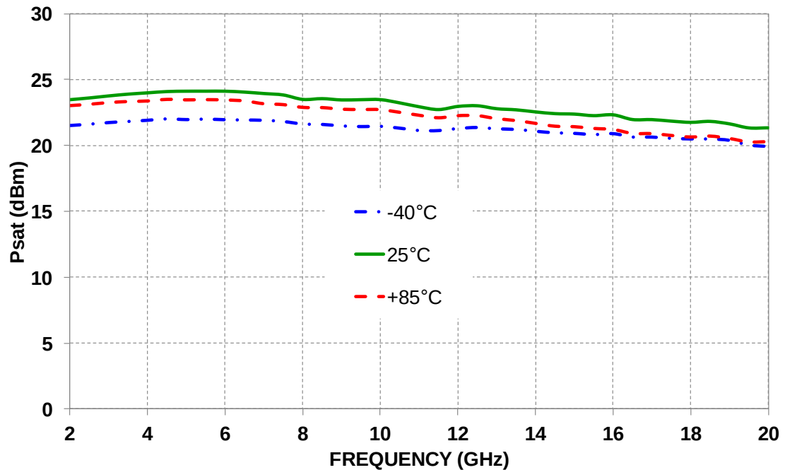
Saturated Output power vs temperature
