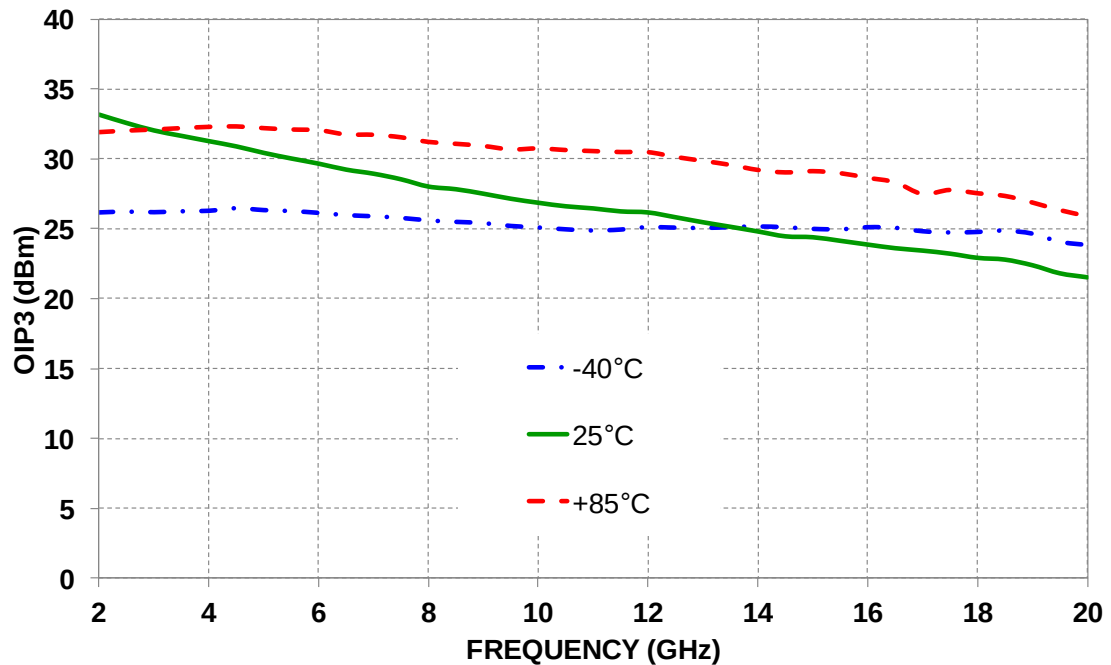
Output IP3 vs temperature
