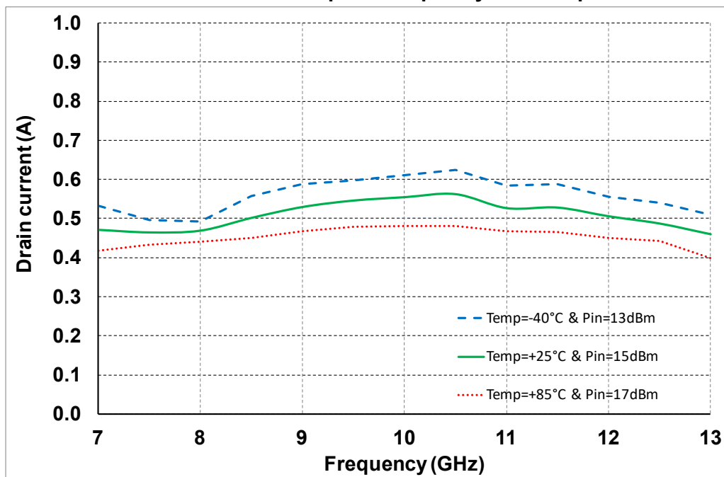
Drain current at 3 dBcomp vs. Frequency and Temperature
