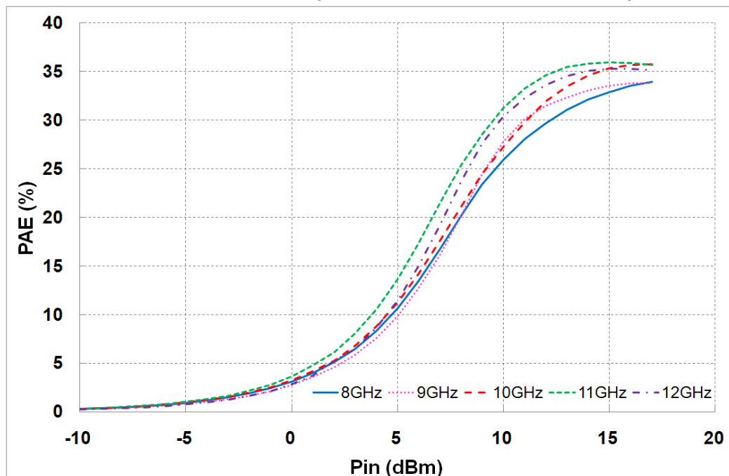
Power added efficiency vs. Input Power and Frequency
