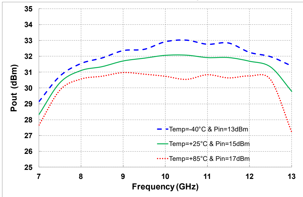
Output Power at 3dBcomp vs. Frequency and Temperature
