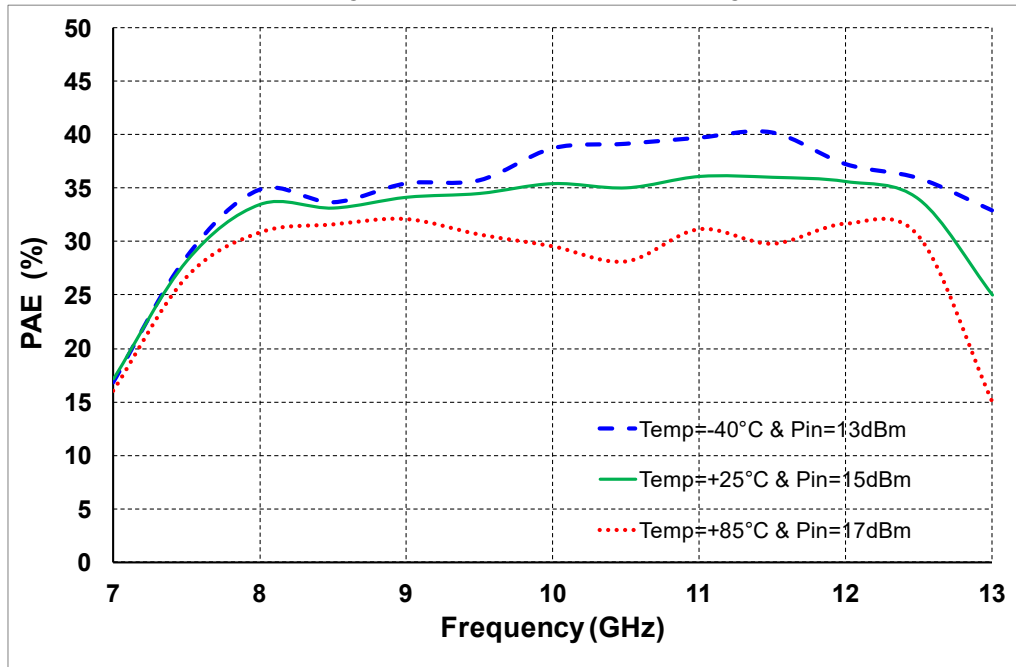
Power added efficiency at 3dBcomp vs. Frequency and Temperature
