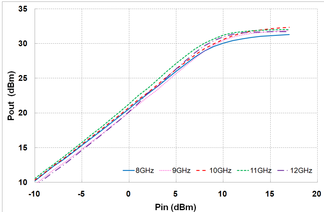
Output Power vs. Input Power and Frequency
