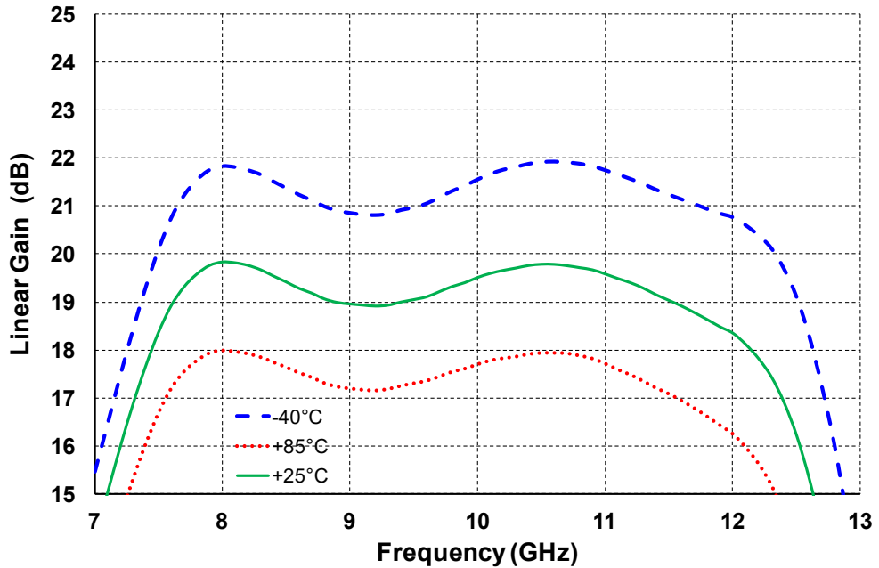
Linear Gain vs. Frequency and Temperature
