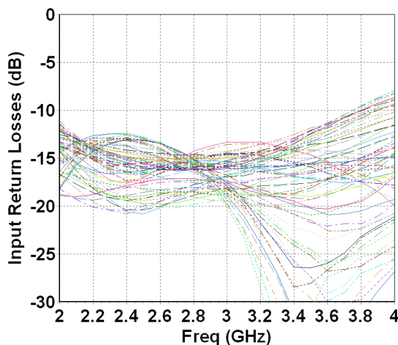
Input Return Losses @ All States
