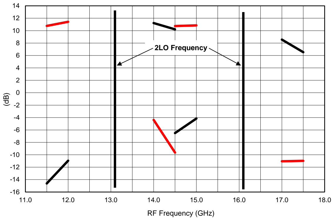
Conversion gain & Image suppression with a 90° IQ combiner @ IF=1 & 1.5GHz
