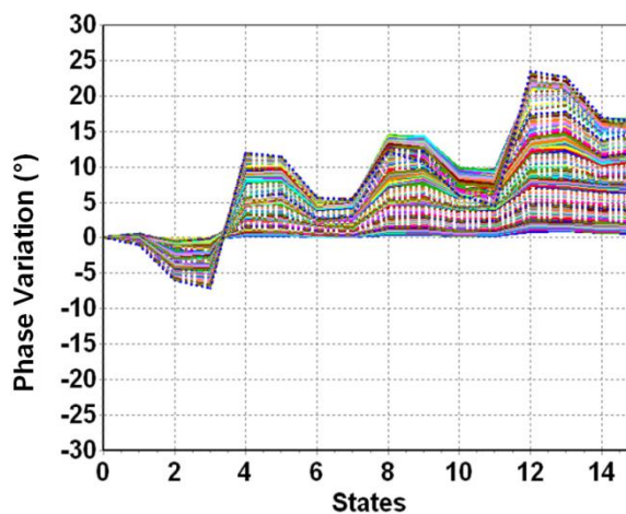
Phase Variation versus States 2GHz < Frequency < 35GHz
