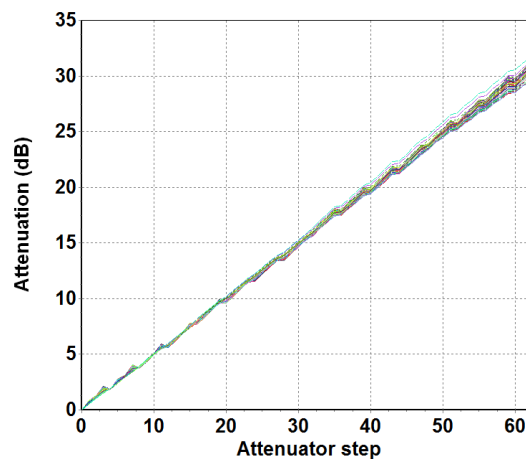
Attenuation versus attenuator state Frequency bandwidth 4-16GHz
